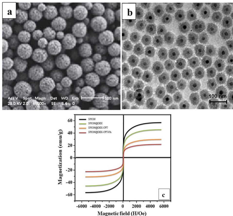
Figure 2: a. transmission electron microscopy (TEM) and scanning electron microscopy (SEM) images of supermagnetic iron oxide nanoparticles (SPIONs). b. supermagnetic iron oxide-dextran-camptothecin-folic acid nanoparticles (SPION-DEX-CPT-FA) nanoparticles showing spherical morphology and coating structure. c. Magnetization curves of uncoated SPIONs and SPION@DEX-CPT-FA obtained by VSM, showing superparamagnetic behavior.
